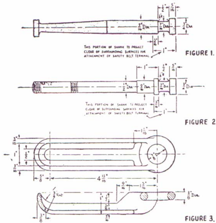
PLATE I ANCHORS AND TERMINALS FOR SAFETY BELTS.
