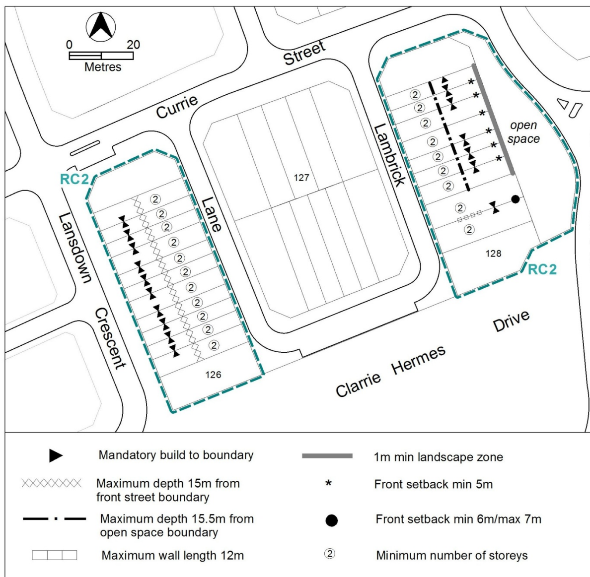
Figure 1 Building Controls
