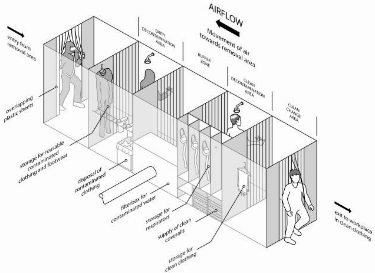
Figure 1: Decontamination unit.
